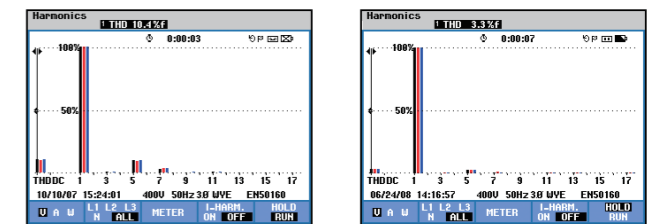
Harmonic spectrum of phase voltages before and after HTQF APFs were installed
