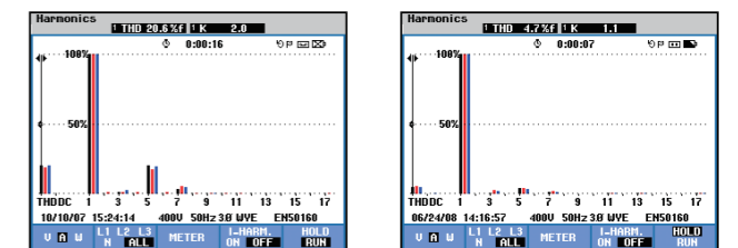
Harmonic spectrum of phase currents before and after HTQF APFs were installed
