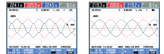
Waveforms and RMS values of phase voltages before and after HTQF APFs were installed
