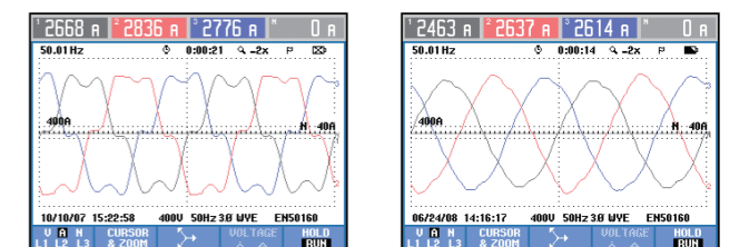
Waveforms and RMS values of phase currents before and after HTQF APFs were installed
